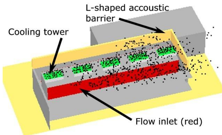
Figure 16. Detailed snapshot with SmokeView of water vapor particles emanating from the cooling towers and reentraining into the flow inlet (shown in red).
