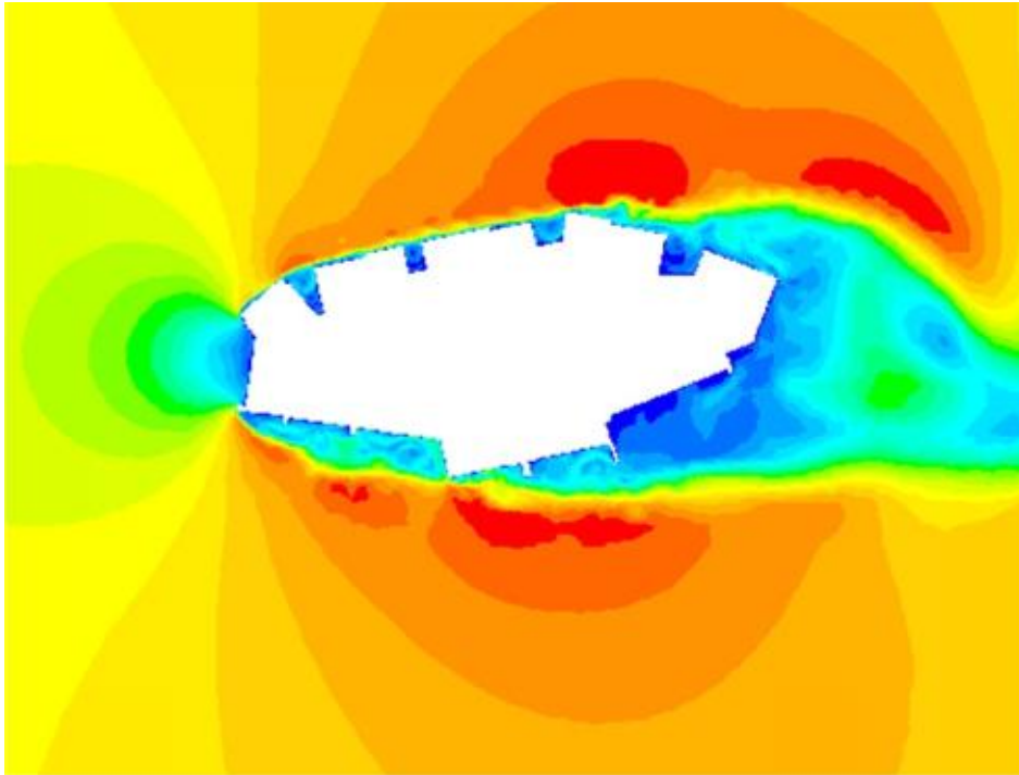
Figure 10. The flow is from left to right in this LES, unsteady, snapshot of the velocity magnitude contours (blue = 0 m/s and red = 15 m/s). This initial design formed a baseline for modifying the building shape to reduce the crosswind response (after CPP Inc.). The full flow video may be seen at www.aawe.org .
