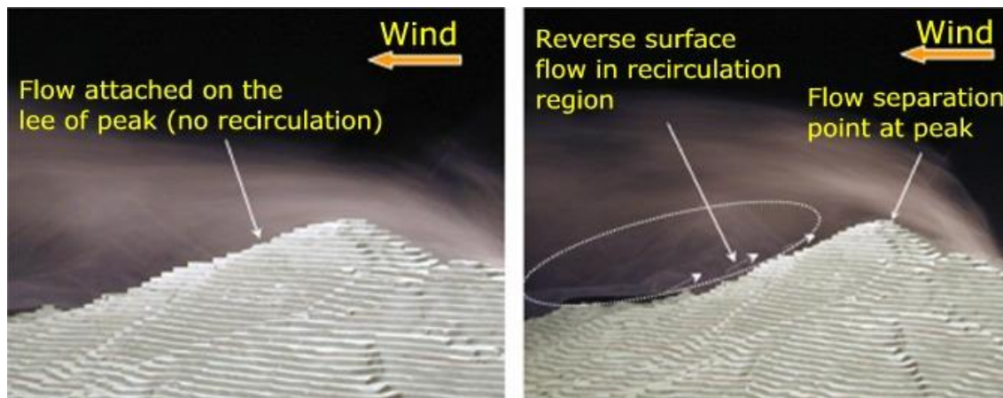
Figure 11. Wind tunnel simulation showing intermittent flow separation and reattachment over a terrain peak on scale model of Lantau Island near Hong Kong. Modeling separation behavior with CFD can be erroneous and lead to misrepresentation of flow downwind of peak as shown by Derickson and Peterka (2004).
