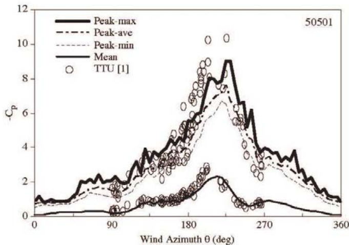
Figure 8. Range of peak pressure coefficients from a model of the TTU Building collected by multiple ergodic experiments in the wind tunnel (after Endo, Bienkiewicz and Ham 2006).
