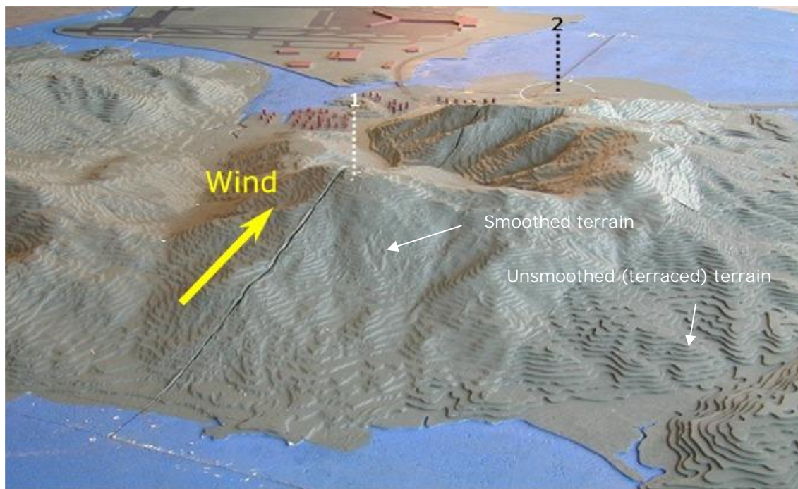
Figure 12. Full view of scale model of Lantau Island near Hong Kong. Point 1 denotes the peak shown in Figure 11. Because of poor representation of intermittent cycles of flow separation and reattachment, the CFD model did poorly in simulating the flow at all locations between Points 1 and 2. Note also the smoothed and terraced portions of the terrain model in the study (from Derickson and Peterka, 2004).
