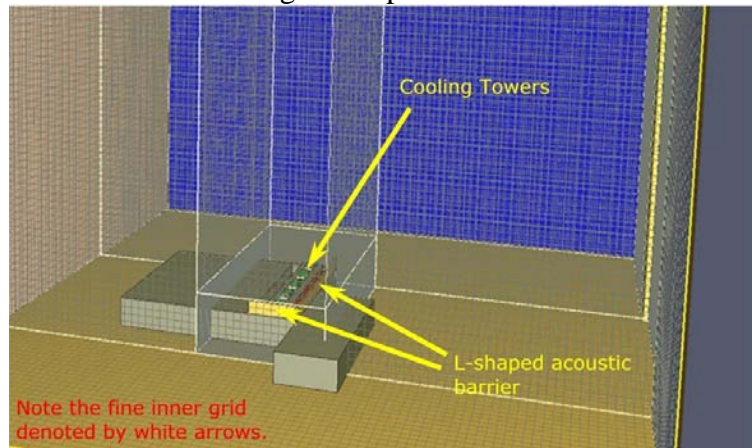
Figure 14. Computational grid to study reentrainment of cooling tower plumes into flow inlets due to addition of an acoustic barrier surrounding the towers on the edge of the building roof. Grid resolution is refined in the vicinity of the acoustic barrier and cooling towers to capture the flow physics accurately.
