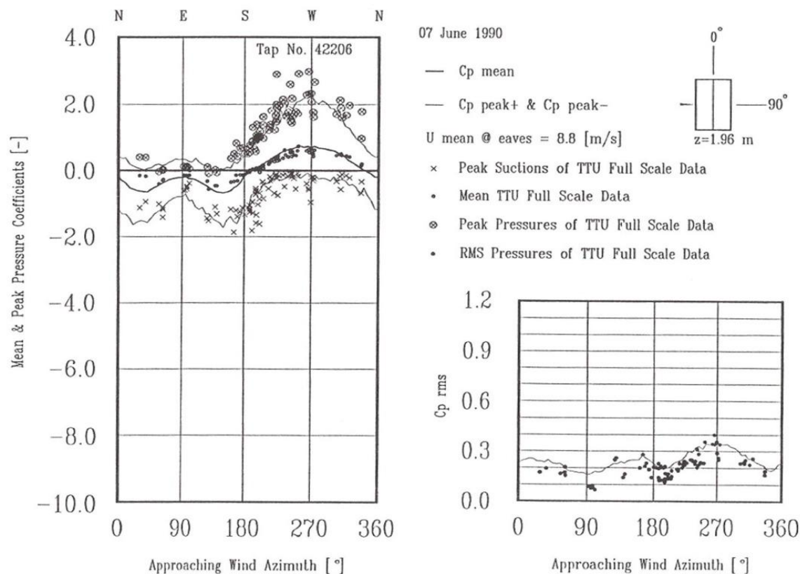
Figure 3. Full-scale and model-scale (1:100) pressure coefficient data for the Texas Tech Building for a tap located at the center of the long wall (after Cochran, 1992).
