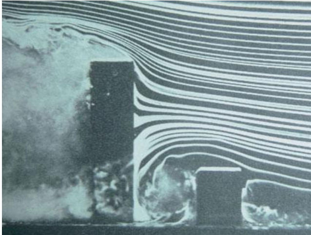
Figure 17. Massively separated flow in the lee of the tall building (after Van Dyke, 1982).
