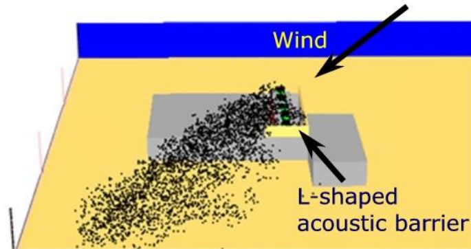
Figure 15. Instantaneous snapshot with SmokeView of particles depicting the transport and dispersion of the cooling tower water vapor plumes. Note direction of wind and location of acoustic fence.
