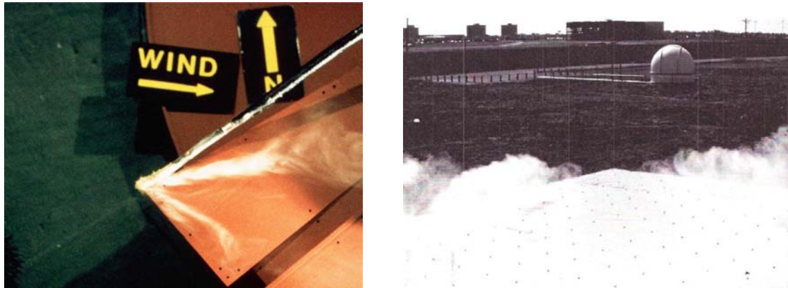
Figure 5. Roof-corner vortices on a wind-tunnel model (left) and on the TTU Building (right).
