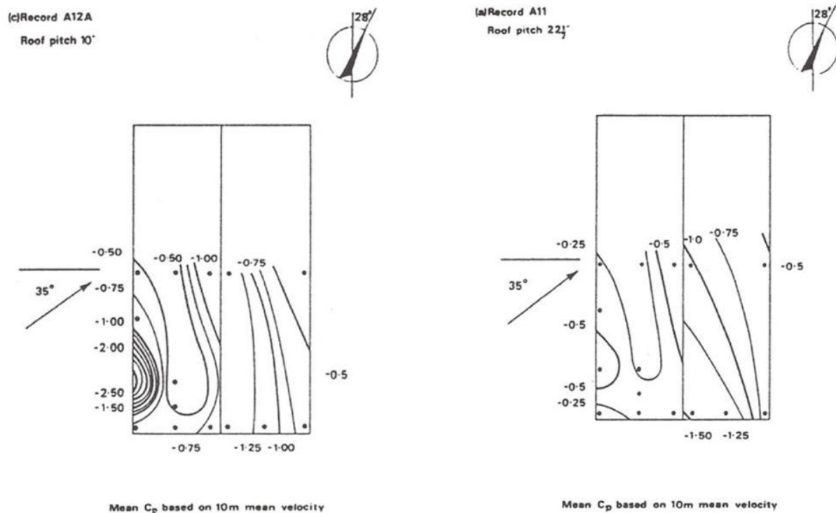
Figure 2. Mean, full-scale, pressure contours for cornering winds on two roof slopes (10 and 22.5 degrees) of the Aylesbury House in Great Britain in the 1970s (after Eaton and Mayne, 1975).
