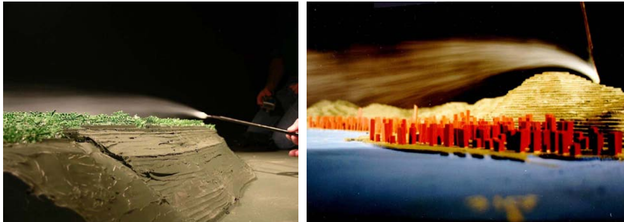
Figure 13. Exploring flow separation on an escarpment model for a potential wind energy project (left) and over Victoria Peak on Hong Kong Island (right) for the wind structure at Central in the boundary-layer wind tunnel.
