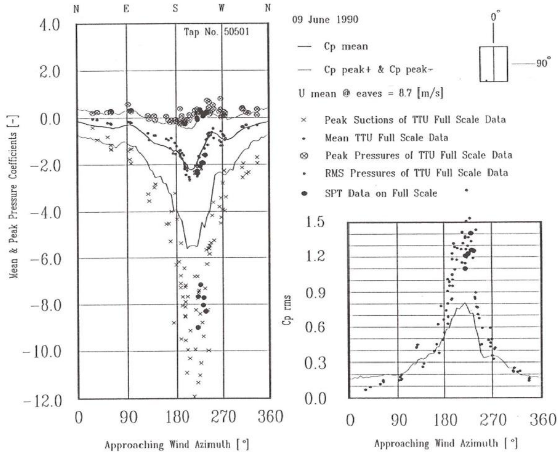
Figure 4. Quartering winds at the roof corners produce roof-corner vortices. Wind-tunnel data do not capture the same magnitude of peak coefficients due to the relative tap size (see SPT data) and Reynolds number influences discussed below (after Cochran 1992).
