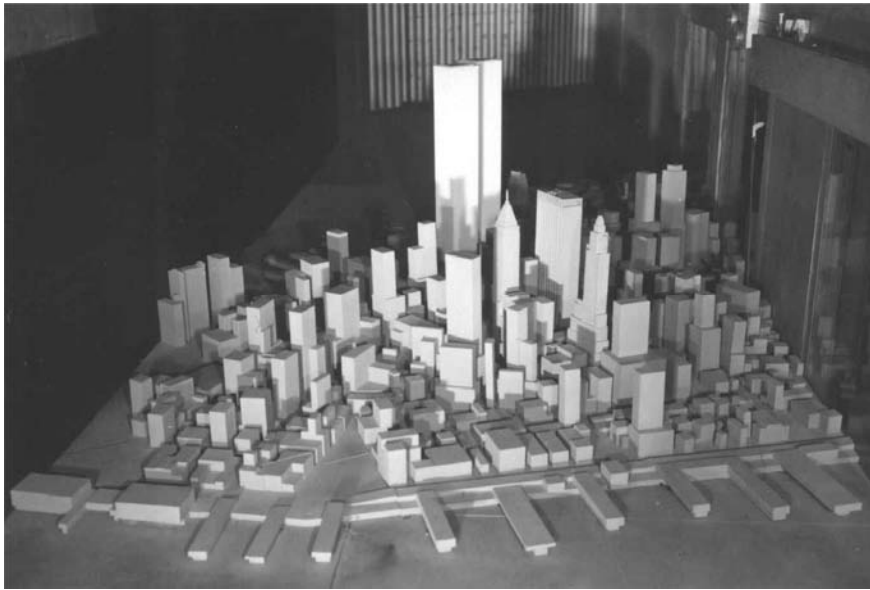
Figure 1. The aeroelastic models of the World Trade Center, with surrounding Manhattan model, in one of the Colorado State University wind tunnels during the 1963/1964 studies.
