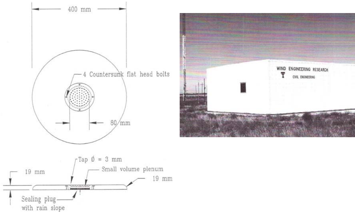
Figure 7. The "super pressure tap" (SPT) used on the TTU Building (right) to illustrate the impact of tap size on the peak data collected. The 80-mm porous-opening diameter corresponds to 0.8-mm value on the 1:100 model.
